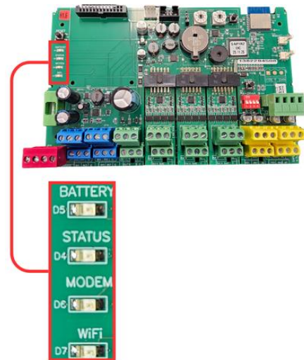
LED'S LOCATION ON THE SAPIR2 BOARD
